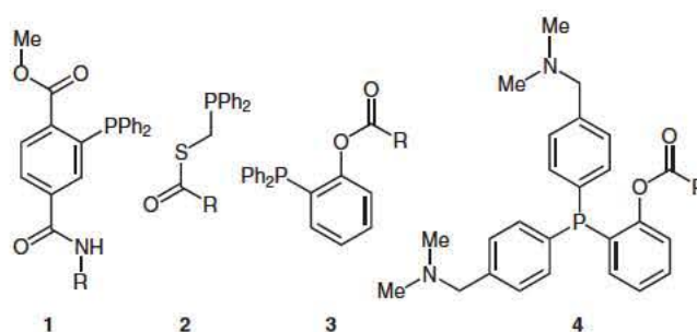
Figure 1 Overview of phosphines for Staudinger ligations
