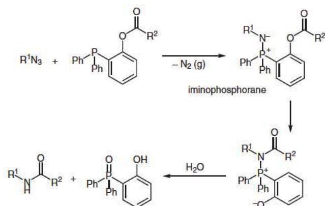
Scheme 1 Putative mechanism of traceless Staudinger ligation
