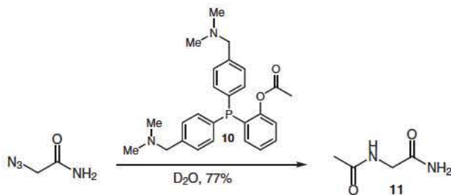
Scheme 3 Investigated traceless Staudinger ligation in water
