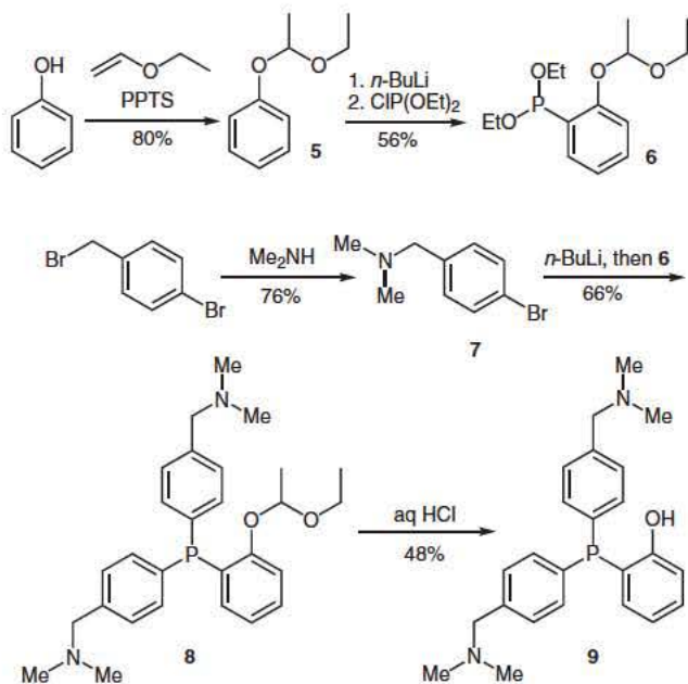
Scheme 2 Synthesis of water-soluble phosphinophenol
