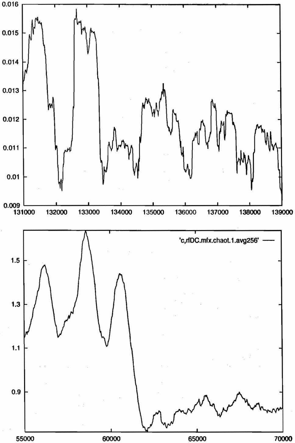
FIG. 4. Rapid changes of brain dynamics can be detected by the chaoticity measures. Cascade of transitions observed via \sigma_{\Lambda} estimated for EEG (90 seconds slice) of schizophrenics (A) and (B) single transition derived from MEG (72 seconds time slice) of tinnitus observed via \Lambda .
