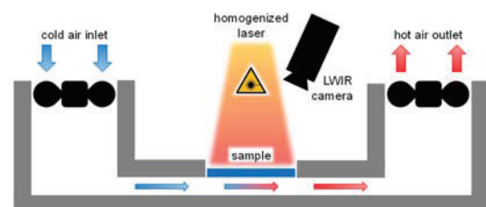
Figure 1: Cross-section drawing of the used wind tunnel.
