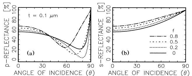
FIG. 4. The results of calculations based on the effective medium theory (Maxwell Garnett) for reflectance vs incident angle for a 0.1 \mu\text{m} thick foamy film on 0.2 \mu\text{m} thick chromium film on a sapphire substrate immersed in water. The optical properties of bulk Cr are used in the calculation [14]. t is the thickness of the foamy liquid film, f is the fractional volume of the bubbles, \lambda_{\text{probe}} = 632.8 nm: (a) p polarized, (b) s polarized.
