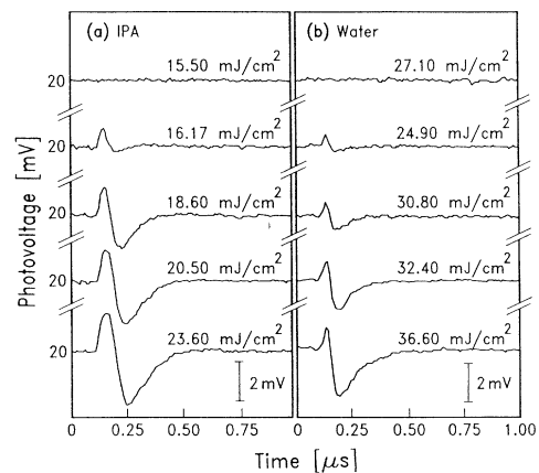
FIG. 2. Transient reflectance signal with increasing excimer laser fluence for 0.2 \mu\text{m} chromium film, \lambda_{\text{probe}} = 752 nm, s polarized, \theta = 7^\circ : (a) IPA, (b) water.
