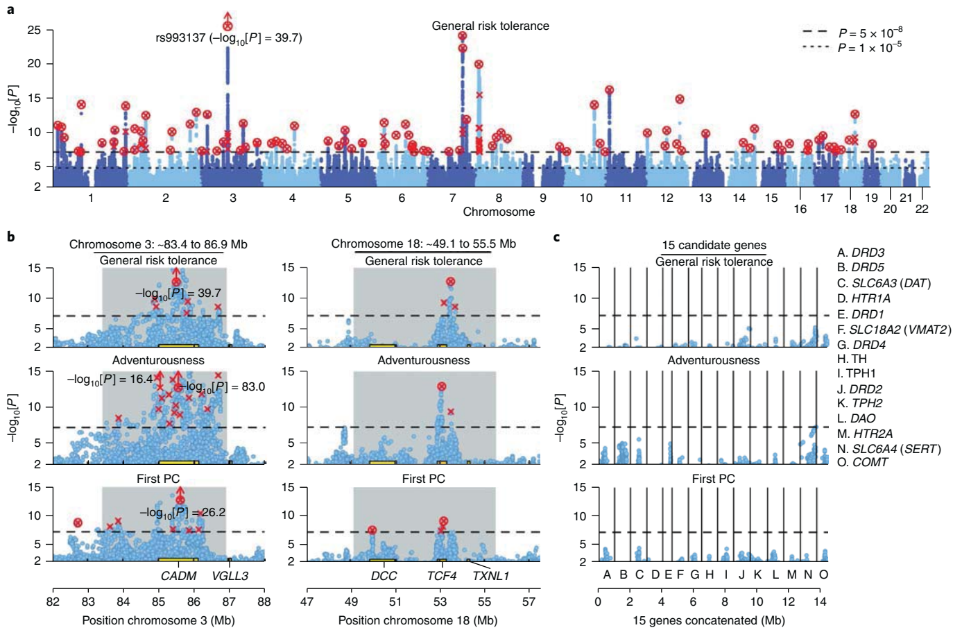
Fig. 1 | Manhattan plots. In all panels, the x axis is chromosomal position; the y axis is the GWAS P value on a -\log_{10} scale (based on a two-tailed z test); each lead SNP is marked by a red x ; each conditional association is marked by a red o ; and each SNP that is both a lead SNP and a conditional association is marked by a red \otimes . a , Manhattan plots for the discovery GWAS of general risk tolerance ( n = 939,908 ). b , Local Manhattan plots of a long-range LD region on chromosome 3 and a candidate inversion on chromosome 18 that contained lead SNPs for all seven of our GWAS. The gray background marks the locations of long-range LD or candidate inversion regions. c , Local Manhattan plots of the areas around the 15 most commonly tested candidate genes in the prior literature on the genetics of risk tolerance. Each local plot shows all SNPs within 500 kb of the gene's borders that were in weak LD ( r^2 > 0.1 ) with a SNP in the gene. The 15 plots are concatenated and shown together in the panel, divided by black vertical lines. The 15 genes were not particularly strongly associated with general risk tolerance or the risky behaviors, as can be seen by comparing the results within each row across b and c (the three rows correspond to the GWAS of general risk tolerance, adventurousness ( n = 557,923 ), and the first PC of the four risky behaviors ( n = 315,894 )).
