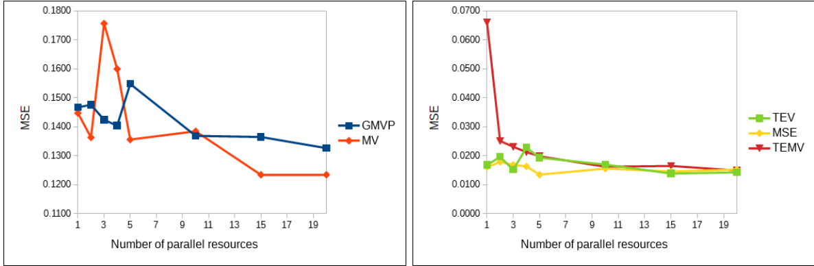
Figure 5.2: Replication of the STOXX50 index with BEAM SEARCH INDEX TRACKING. Tracking portfolio performance while increasing the number of parallel resources. \text{MSE} \times 10^4 versus the search width k .
