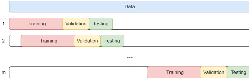
Figure 5.1: Design of the experiment
