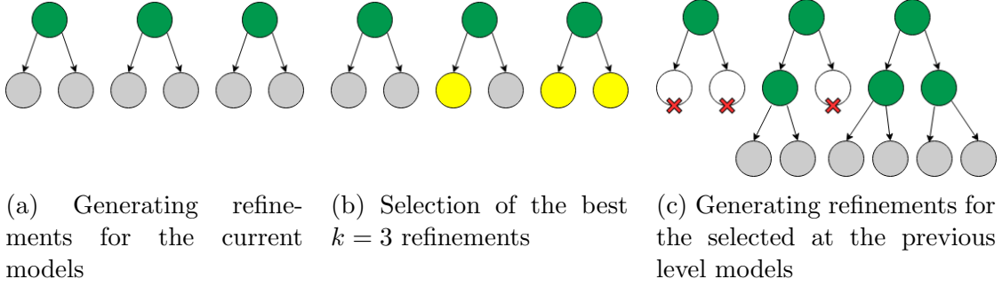
Figure 4.2: The refine-and-select process for BEAM SEARCH with width k = 3
