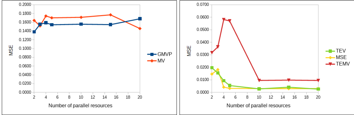
Figure 5.4: Replication of the STOXX50 index with WIDENED INDEX TRACKING. Tracking portfolio performance while increasing the number of parallel resources. \text{MSE} \times 10^4 versus the search width k .
