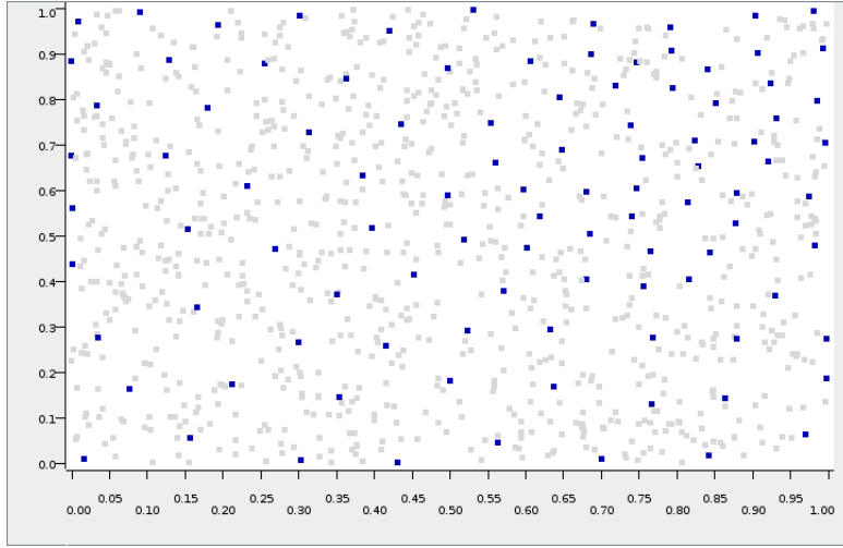
Figure 4.6: A subset of 100 points taken from a set of 1,000 randomly distributed points, representing a near-optimal solution for the p -DISPERSION-MIN-SUM problem
