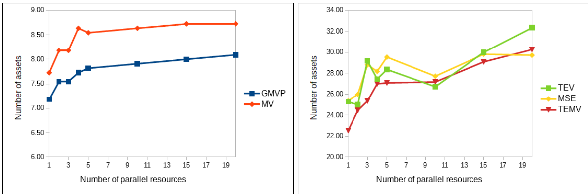
Figure 5.3: Replication of the STOXX50 index with BEAM SEARCH INDEX TRACKING. The number of assets in the tracking portfolio p while increasing the number of parallel resources (the search width k ).
