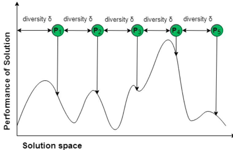
Figure 1.1: Diversity-driven solution space exploration. Inducing a diversity measure \delta between solution paths (between portfolios) can help to explore disparate regions of the solution space.
