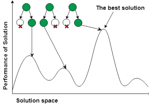
Figure 4.4: DIVERSITY-DRIVEN WIDENING. Inducing a diversity measure between solution paths can help to explore disparate regions of the solution space.
