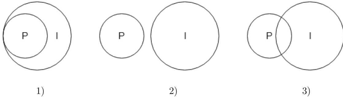
Figure 2.1: Structure of the sample universe. P is a set of assets in the tracking portfolio, I is a set of index constituents. 1) The tracking portfolio P is a proper subset of the index I . 2) The tracking portfolio P and the index I are disjoint subsets. 3) The tracking portfolio P contains some elements of the index I .
