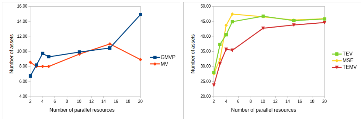
Figure 5.5: Replication of the STOXX50 index with WIDENED INDEX TRACKING. The number of assets in the tracking portfolio p while increasing the number of parallel resources (the search width k ).
