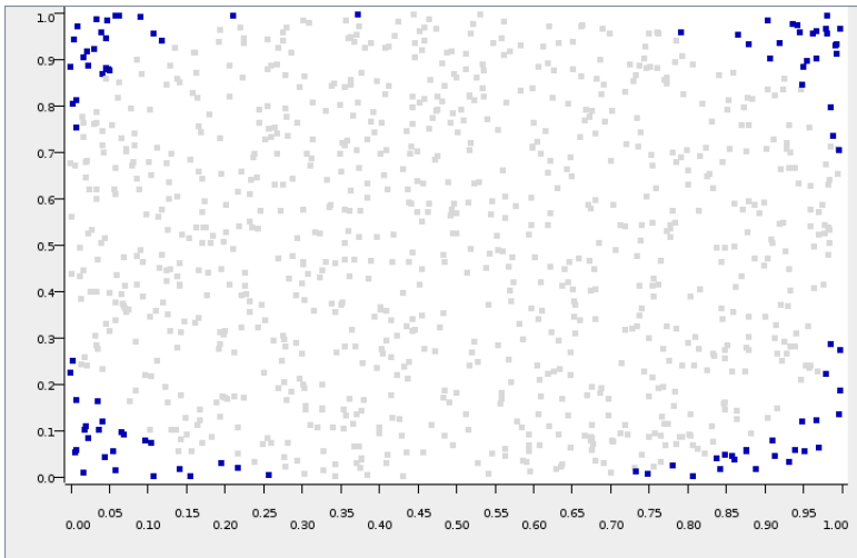
Figure 4.5: A subset of 100 points taken from a set of 1,000 randomly distributed points, representing a near-optimal solution for the p -DISPERSION-SUM problem
