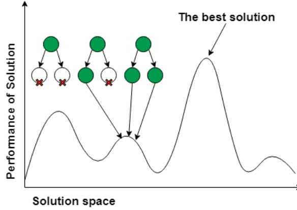
Figure 4.3: Exploitation effect of BEAM SEARCH. Obtained by BEAM SEARCH solutions can be closely related variations of one model.
