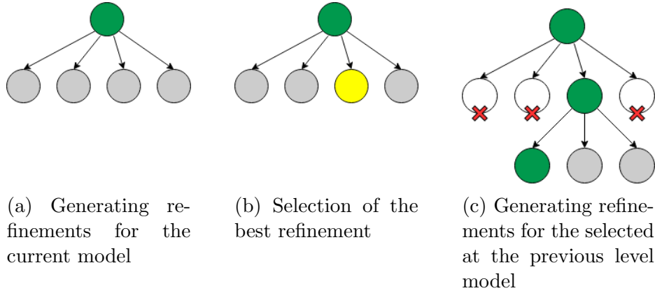
Figure 4.1: The refine-and-select process for the HILL-CLIMBING algorithm
