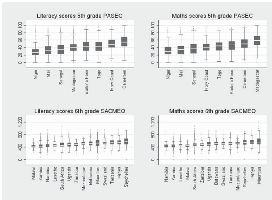
Figure 1. Boxplots of student outcome measures across countries.
