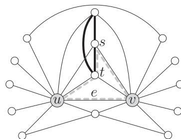
Fig. 2. Triangles at edge e [17,20] do not capture mediator edges (bold), while quadrangles do.
