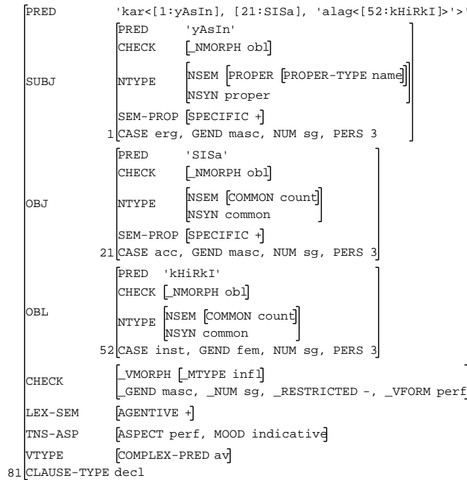
Figure 4: LFG dependency (f-structure) analysis for (9)
